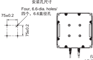
Mounting Hole Dimensions/ 安装孔尺寸
