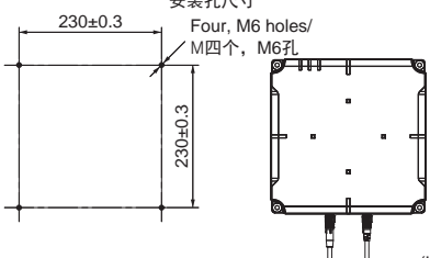
Mounting Hole Dimensions/ 安装孔尺寸
